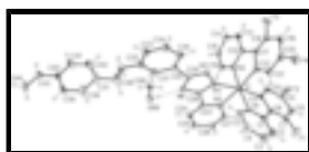
Fig. 1. Structure of the title complex. Displacement ellipsoids represent 50% probability levels. The dashed line represents the classical H bond H99...N6. The minor disorder component is omitted.
